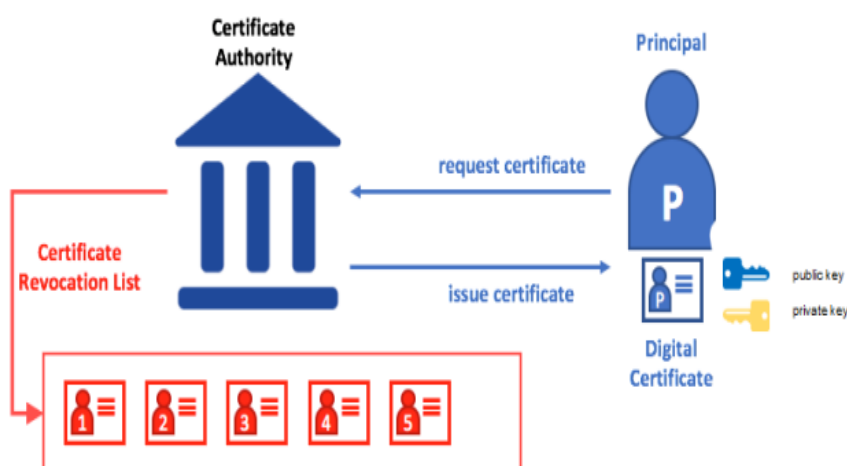
Figure 3 - Certificate Authority.
