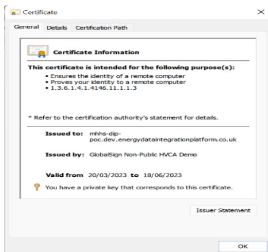
Figure 1 - Digital Certificate.
