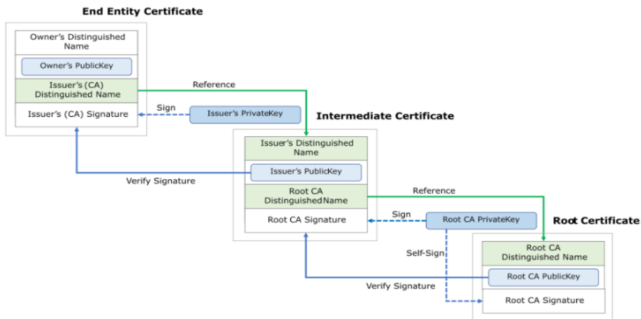
Figure 4 - Certificate Chain.
