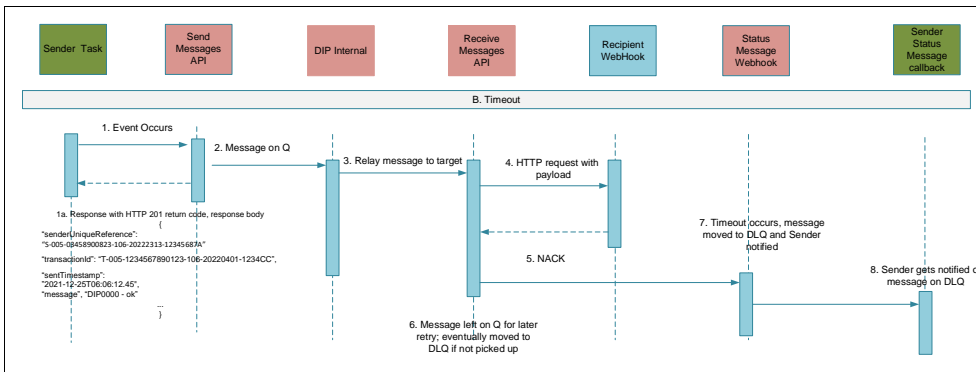
Figure 12 – Recipient Timeout
